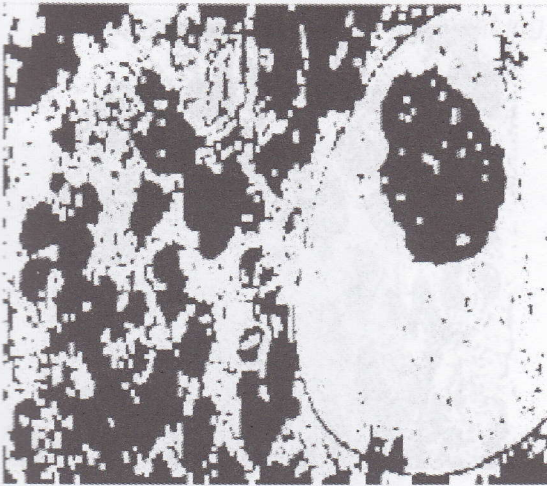
Gambar. 51. Erosion
