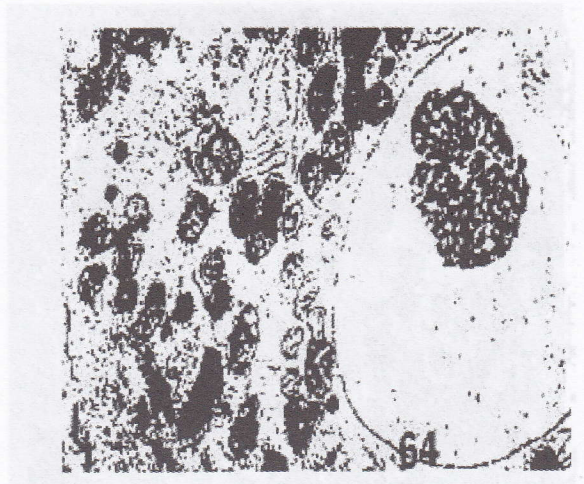
Gambar 51. Erosion
