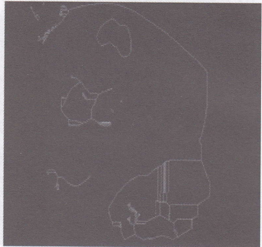
Gambar. 18. Shrink
