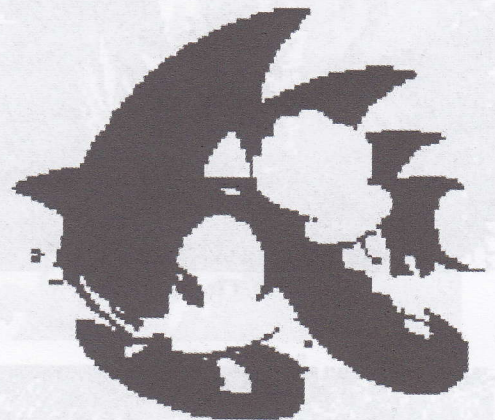
Gambar. 36. Binary Image
