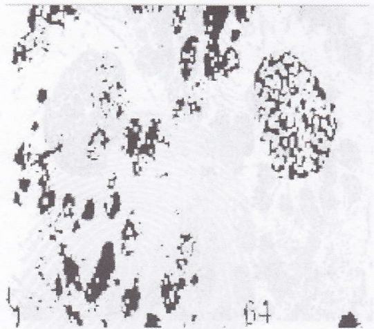
Gambar. 52. Dilation
