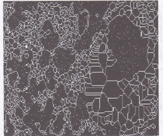
Gambar 53. Morphological Opening
