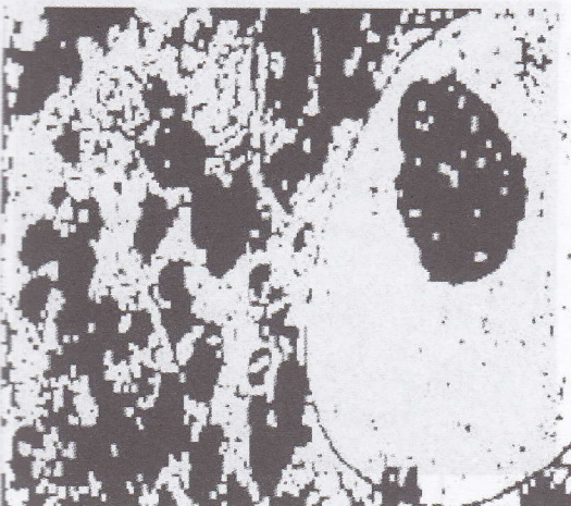
Gambar. 53. Morphological Opening
