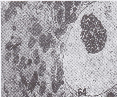
Gambar. 49. Original Image
