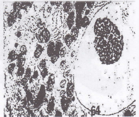
Gambar. 50. Binary Image
