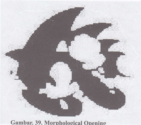
Gambar. 39. Morphological Opening
