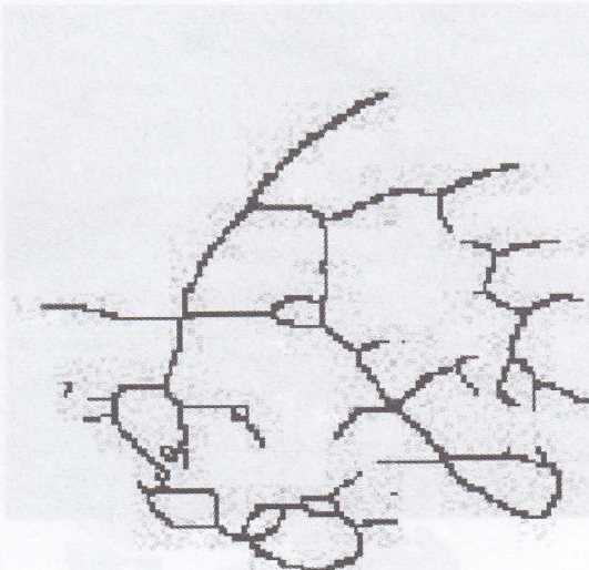
Gambar. 47. Thicken
