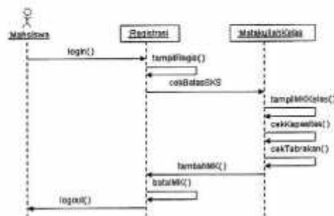
Gambar 5. Sequence Diagram Sistem
