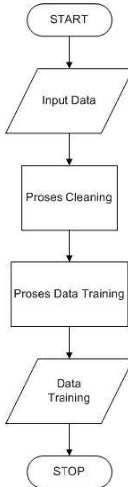
Gambar 2 Pre Processing
